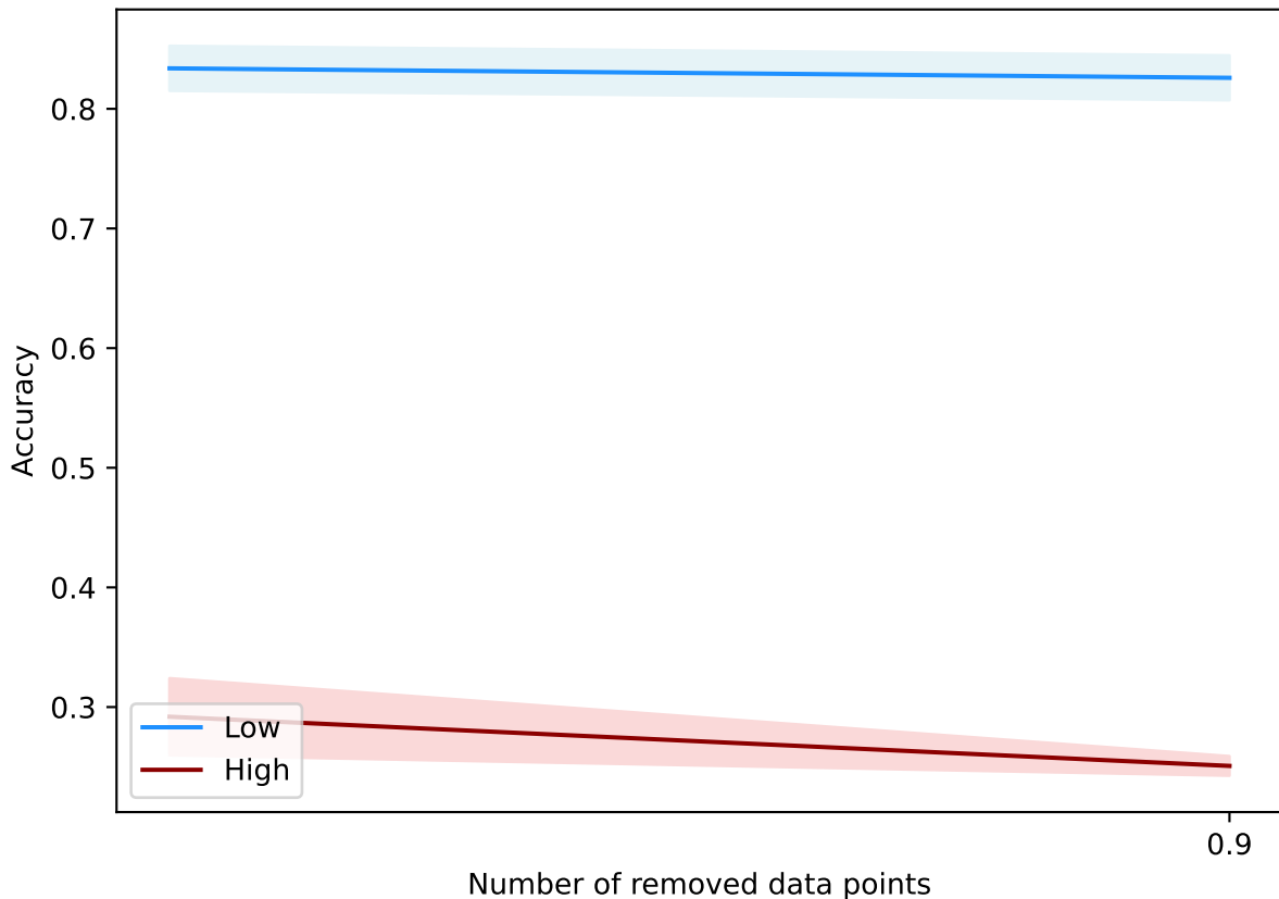
DataAttrOpt(10000, 0.02, 15, best, +b, alpha=best) - nomao
